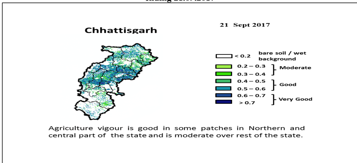
Normalized Difference Vegetation Index (NDVI) Map for Chhattisgarh state for week ending 21.09.2017
